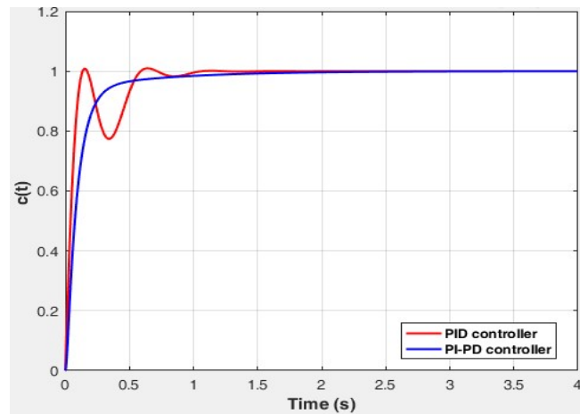
Figure7: Unit Step Time Response using a Tuned PI-PD Controller.
