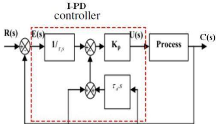
Figure2: I-PDControlledProcess[3,11].
