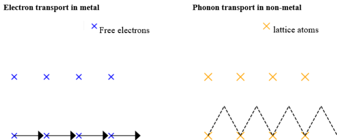
Figure 1. The mechanisms of heat transfer in various materials, such as the movement of electrons in metals and the transport of phonons in non-metals.
