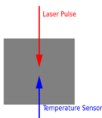
Figure 3. Laser flash analysis, transient planar source, transient hot wire technique
