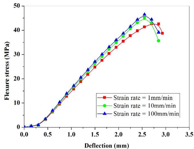
Figure 4. Flexure Stress–deflection Curves of NHS4 Sandwich Panels
