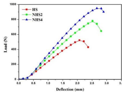
Figure 1. Flexure Load-deflection Curves of HS, NHS2 and NHS4 Sandwich Panels
