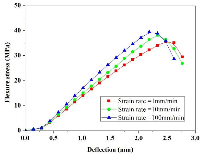
Figure 3. Flexure Stress–deflection Curves of NHS2 Sandwich Panels
