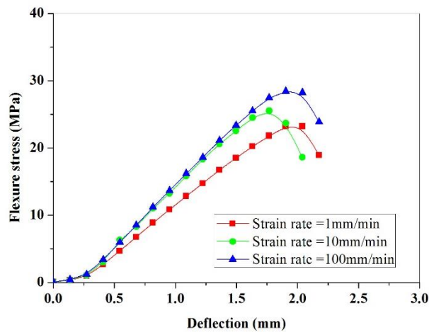
Figure 2. Flexure Stress-deflection Curves of HS Sandwich Panels
