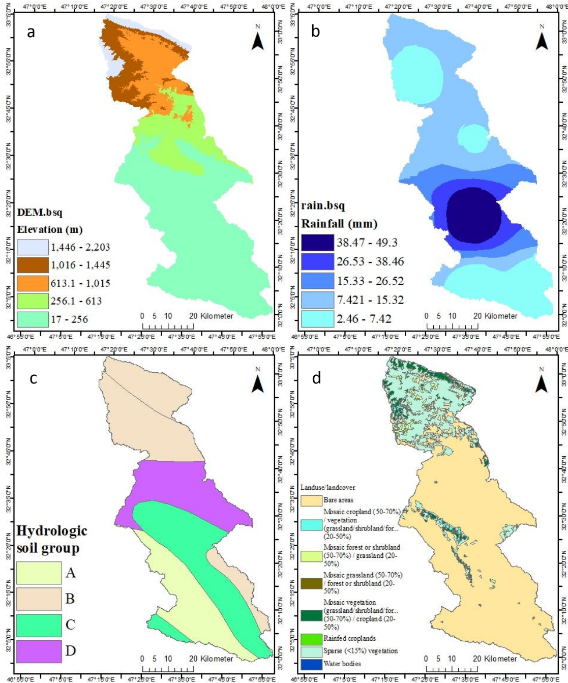
Figure 2: a). SRTM-DEM data, b). rainfall storm, c). Hydrological soil groups, and d) LULC map.
