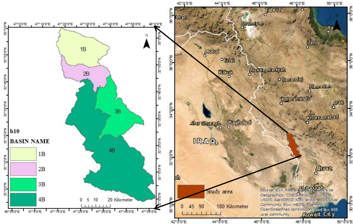
Figure 1: Location map of al-dworeeg valley basin
