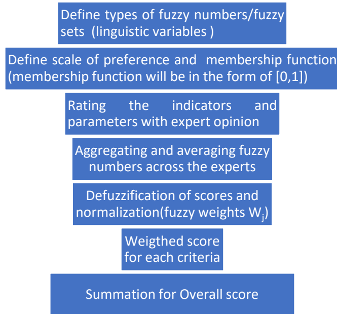
Figure 1: Fuzzy Methodology
