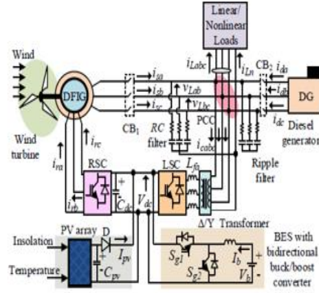
Fig. 1. DFIG based microgrid.
