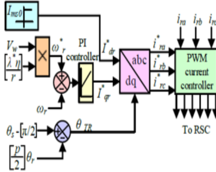
Fig.2. RSC control algorithm.
