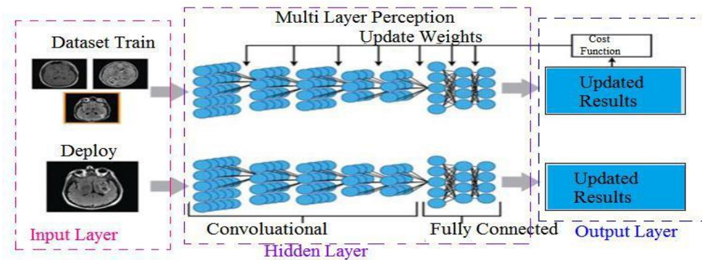
Figure 4. The architecture of the Multi-Layer Perception network
