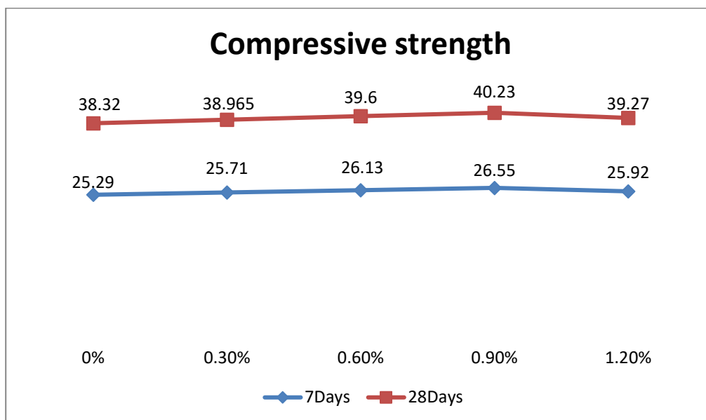
Graph: 3.3: Compressive strength of M30 concrete with optimum % of metakaolin and varying the % of polypropylene fiber
