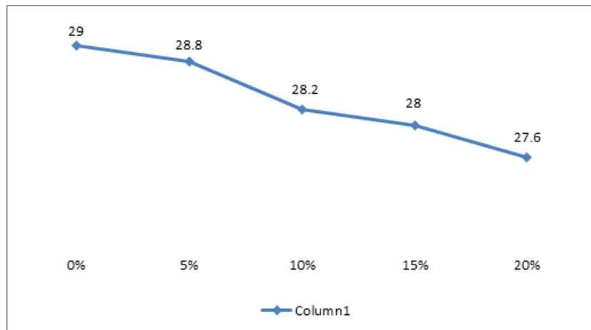
Graph: 3.1: Slump cone test
