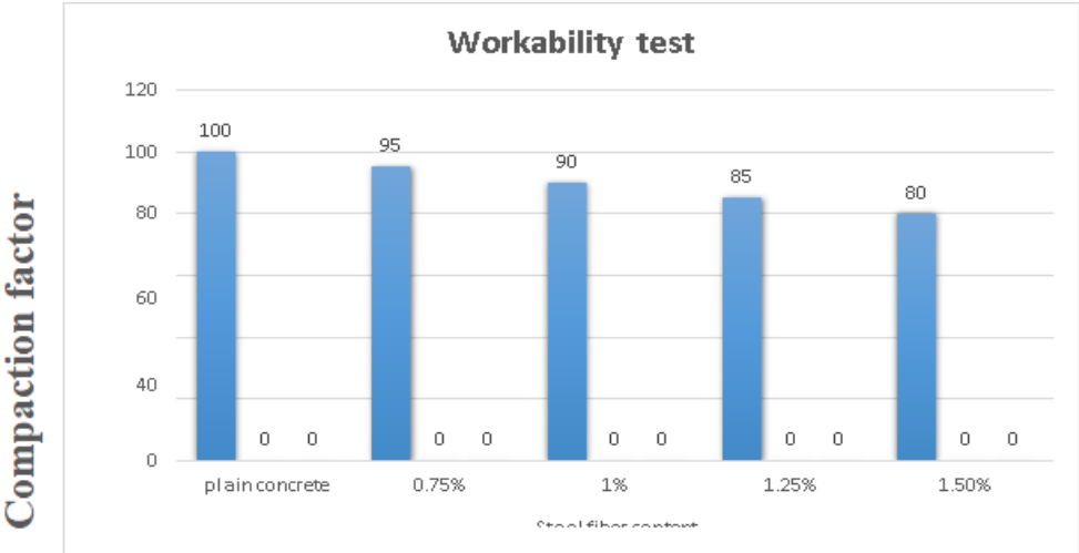
Graph 5.1. Slump cone test result for varying steel content
