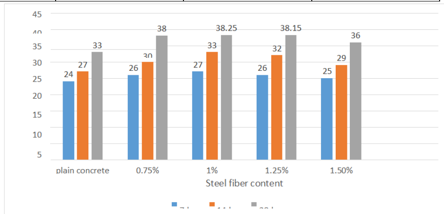
Graph 5.3. Compressive strength test for varying steel content
