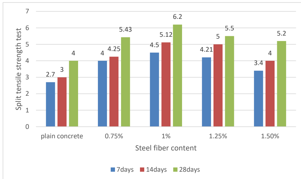
Graph 5.4. Split tensile strength test for varying steel content
