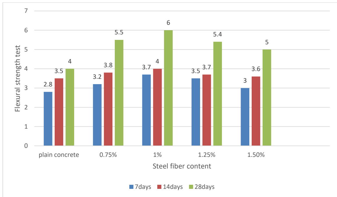
Graph 5.5. flexural strength test result for varying steel fiber content
