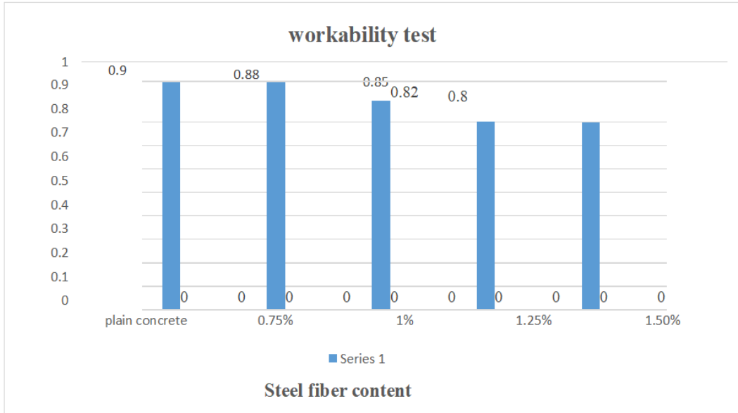
Graph 5.2. Compaction factor test result for varying steel fiber content
