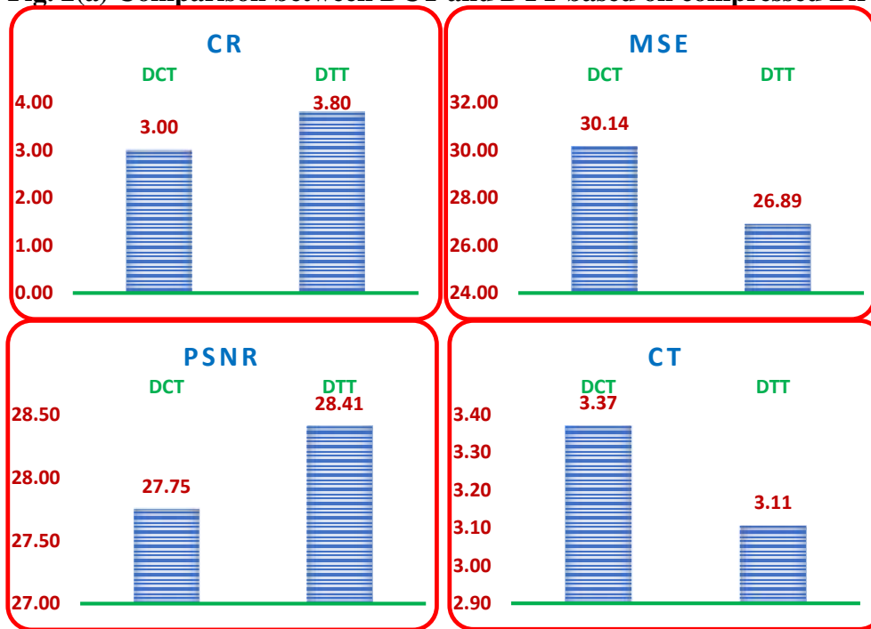
Fig. 2(a) Comparison between DCT and DTT based on compressed Birds images
