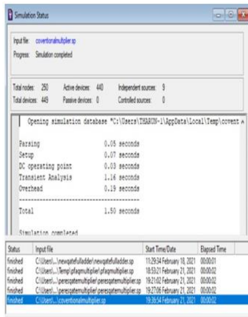
Fig 1: Transistor count output for conventional multiplier circuit
