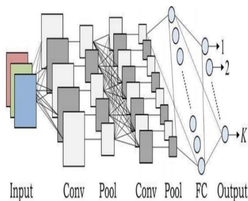
Figure 4: CNN Architecture
