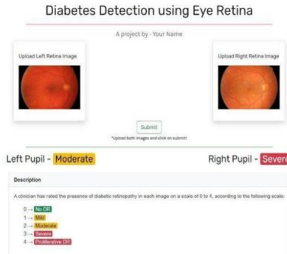
Figure 6: GUI of the implemented system
