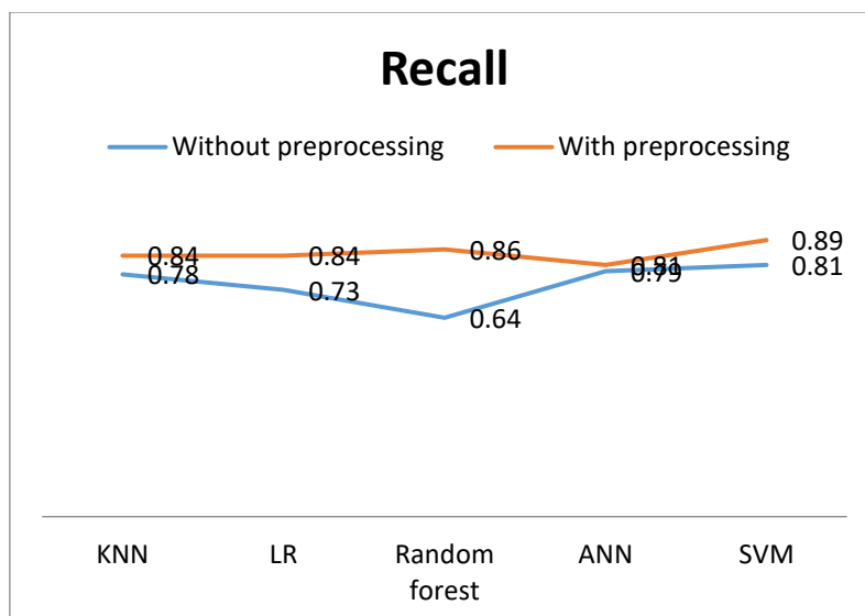
Figure 6: Graphical Representation of Recall of with and without preprocessing stage
