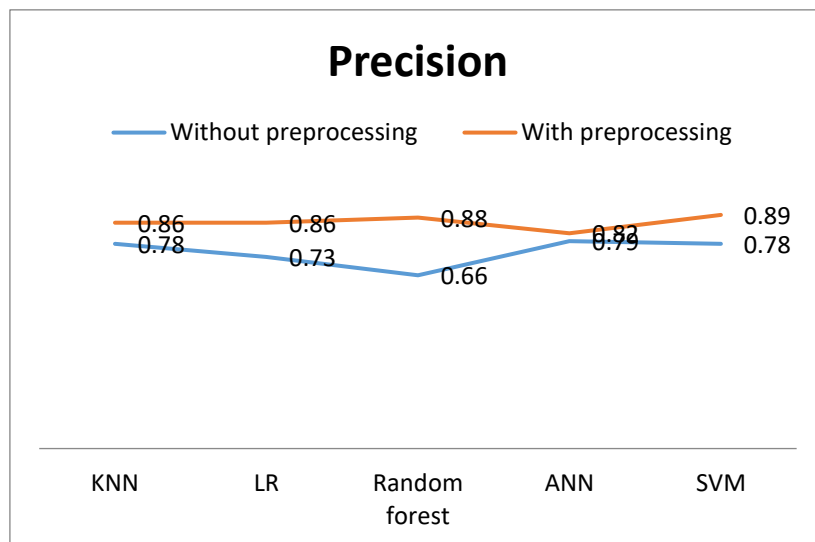
Figure 5: Graphical Representation of Precision of with and without preprocessing stage
