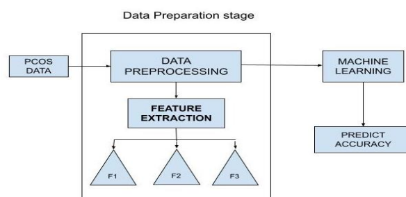
Figure 3: Research Methodology
