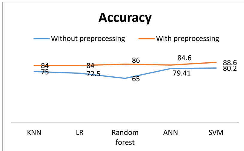
Figure 4: Graphical Representation Accuracies of with and without preprocessing stage
