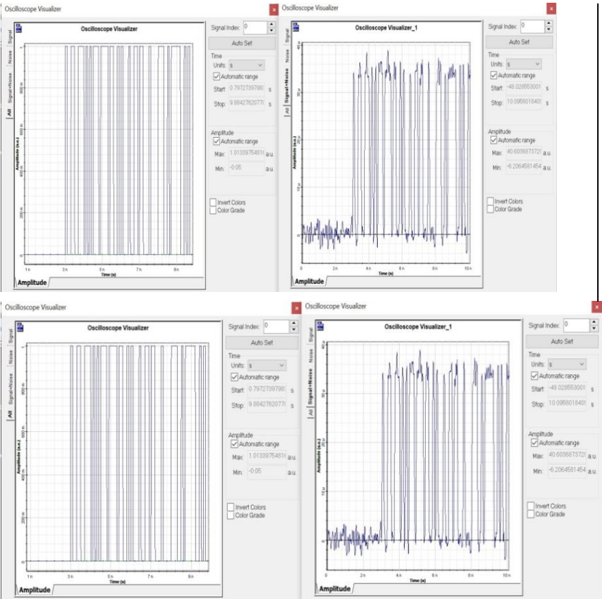
Fig.3:. Transmitted and received signals for ASK
