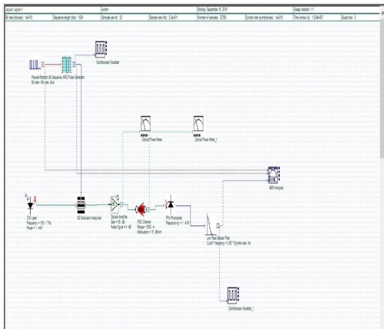
Fig.2: Simulation layout for ASK modulation.
