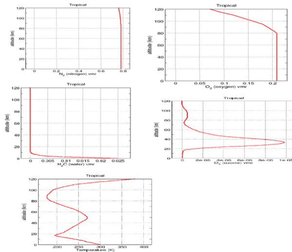
Fig.1: Volume mixing ratio (VMR) of gaseous components Differ with altitude
