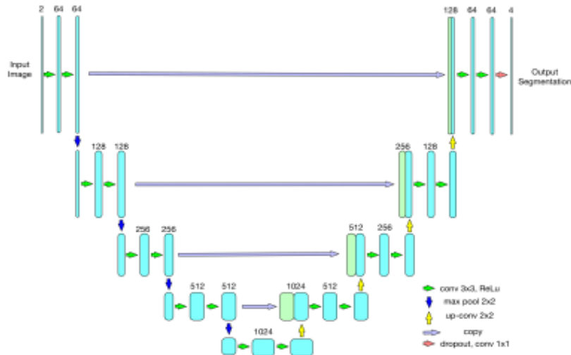
Figure 2. FCN Architecture [29]
