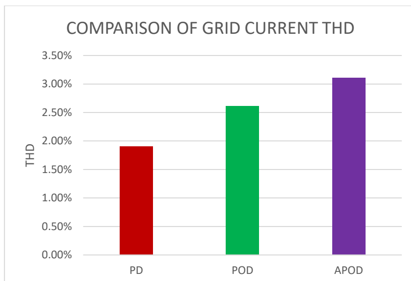
Fig 16 Comparison Of Grid Current Thd
