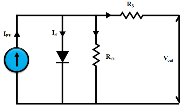
Fig 2electrical Equivalent Circuit Of Pv Cell
