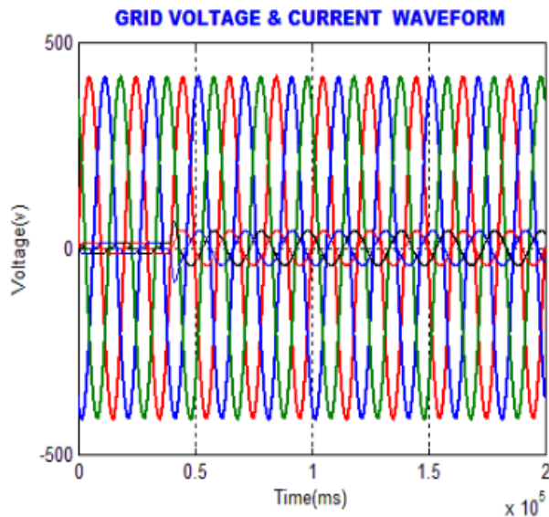
Fig 12 Grid Voltage And Current Waveform
