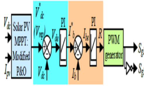
Fig. 6. Control of bidirectional buck or bidirectional boost converter.
