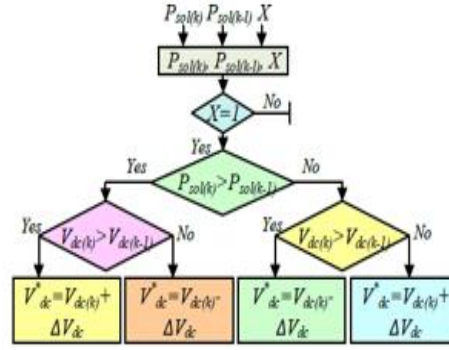
Fig.5. MPPT algorithm of solar PV array.
