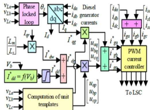
Fig. 3. LSC control algorithm.
