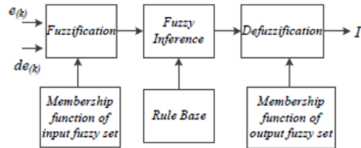
Fig. 9 Structure of Fuzzy Logic Controller
