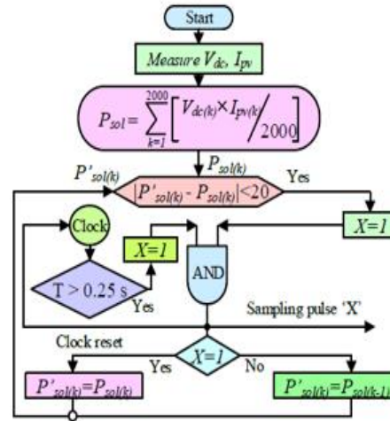
Fig. 4 Sampling pulse generation.
