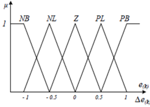
Fig. 8(a) Membership Function of FLC for the input variables
