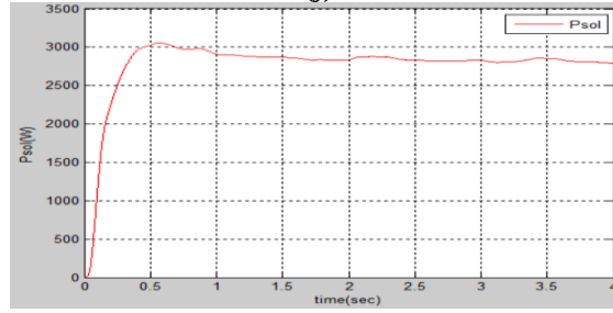
Fig. 10. Performance of bidirectional buck/boost converter at change in load “(a-k)” PL , PLSC , V_{dc} , I_b and V_b , V_r , f_L , \omega_r , PD , P_w and P_{sol} .
