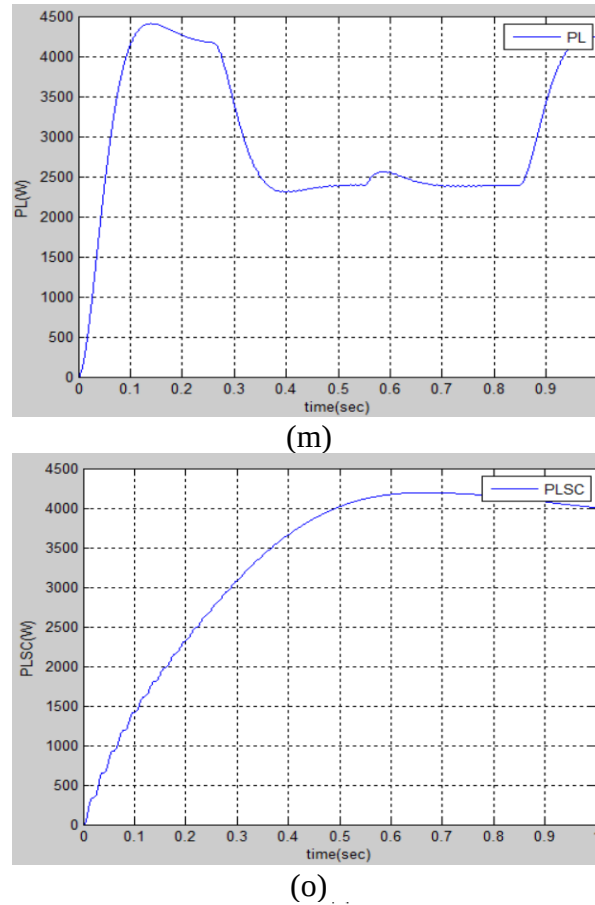
Fig.13. System performance at nonlinear unbalanced load: V_r , V_{dc} , I_b , P_{sol} , P_w , P_D , P_L and PLSC .
